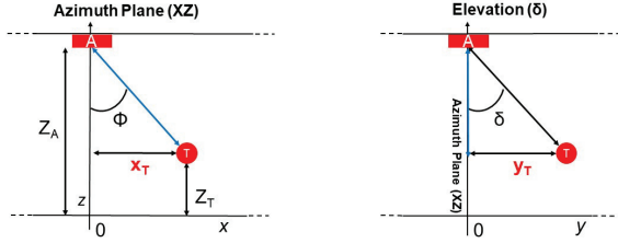
Fig. 4: Computing the coordinates of the tag T in layout 1.
