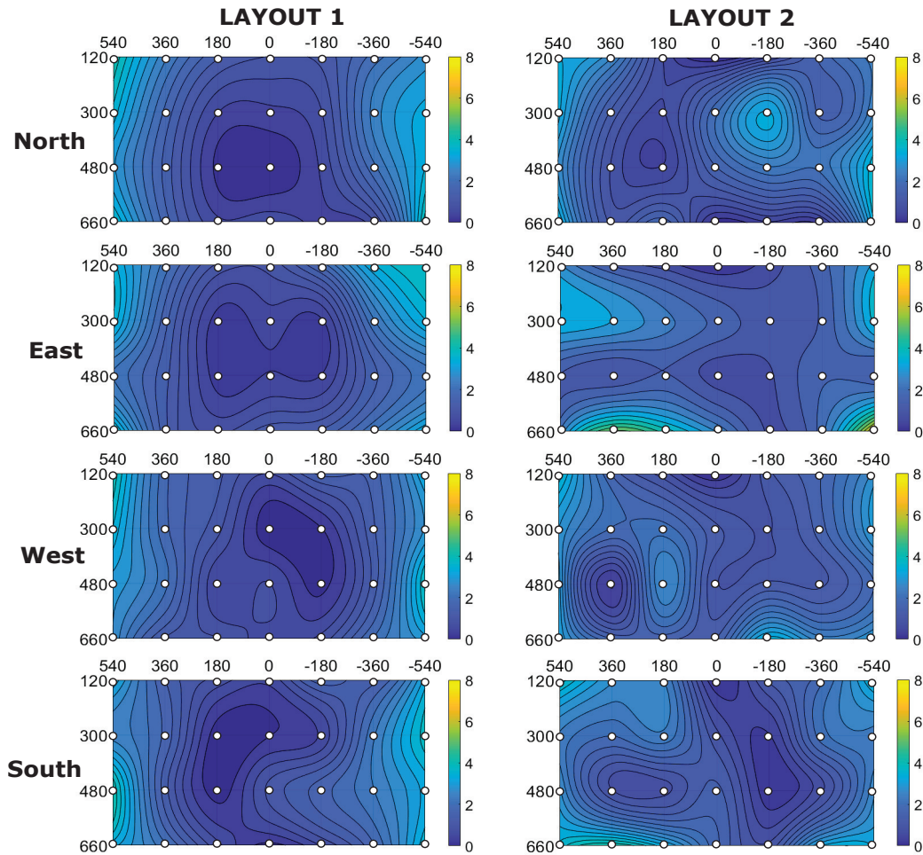
Fig. 6: Localization error \rho expressed in meters for each layout and for different orientations.
