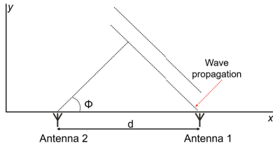
Fig. 1: AoA computation based on the geometry of the antenna array.
