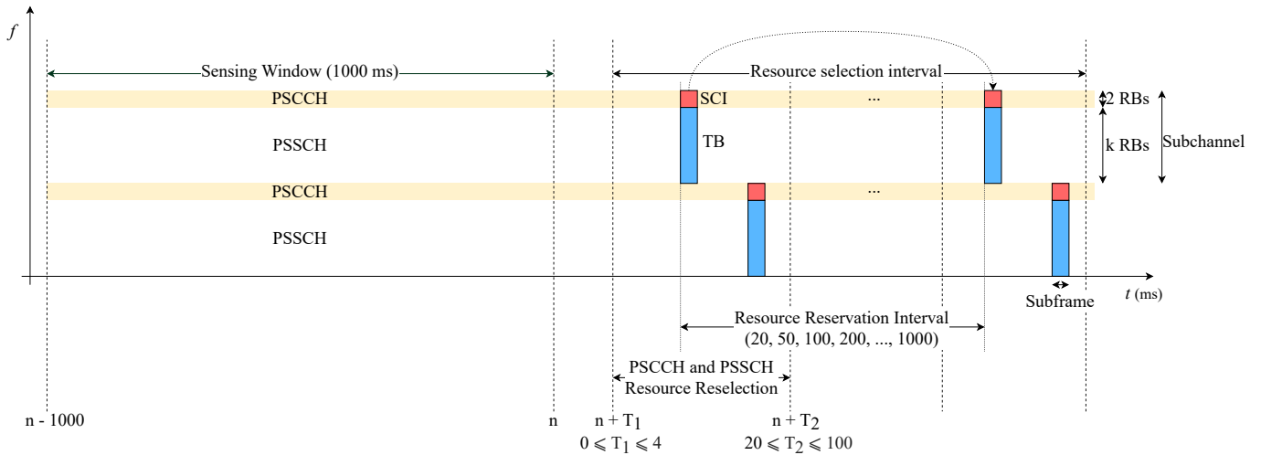
Figure 3: UEs autonomous sensing and resource selection.
