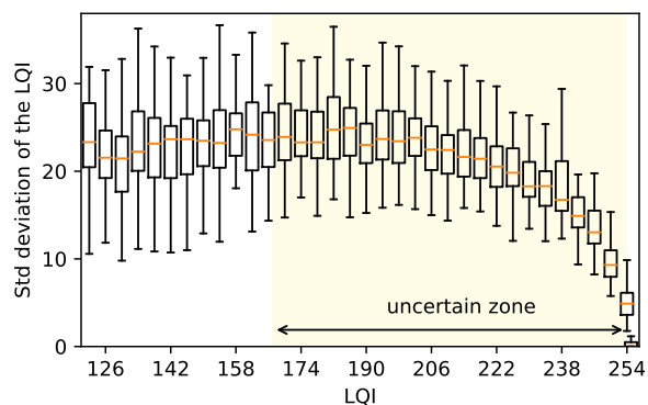
Fig. 5: Variability of LQI. Only links that offer average RSSI \leq -91 dBm are considered and the standard deviation is computed independently on every link.
