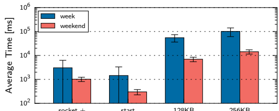
(a) Time measurements for a 2G connection.
