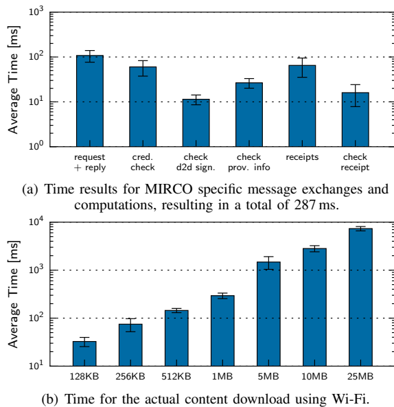
Fig. 4. Time measurements for the respective steps of a content exchange using a D2D connection realized via Wi-Fi. Values shown are the average and the standard deviation. Please note the logarithmic scale.
