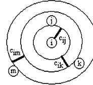
Figure 2. Costs for the mathematical formulation IP .
