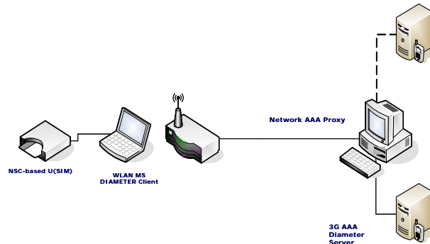
Fig. 7. Testbed for our architecture.
