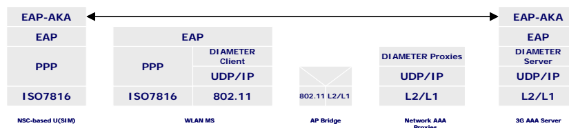
Fig. 3. Our NSC-based AAA protocol architecture in 3G/WLAN interworking.
