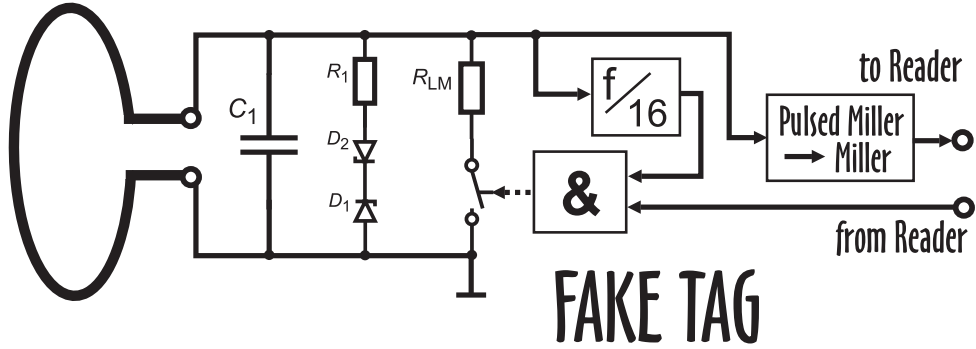
Fig. 4. Operation Principle of the Fake-Tag
