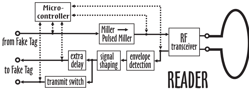
Fig. 3. Operation Principle of the RFID-Reader
