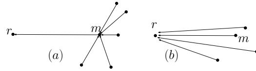
Fig. 7. An example of two possible optimal configurations in CGFP.
