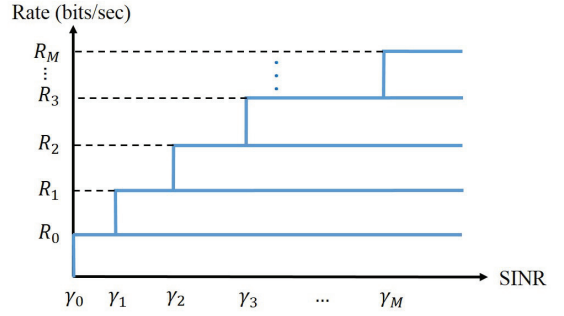
Fig. 1: Rate vs. SINR relationship.
