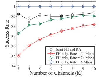
Fig. 3: Success rate vs. K .
