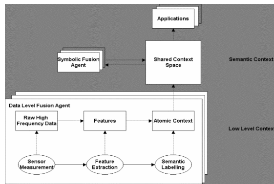
Fig. 2. Context Data Acquisition, Fusion, and Distribution
