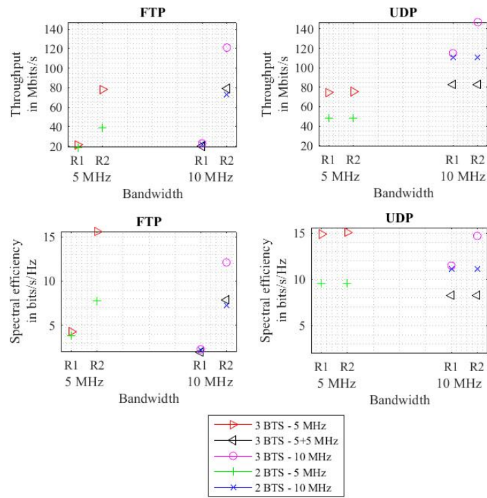
Fig. 5. Variation in the network throughput and spectral efficiency performance between small and large bandwidth usage in the low transmitted power case.
