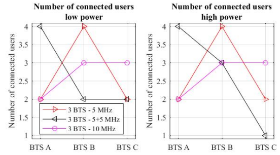
Fig. 4. Number of users connected to each BTS in cases where all 3 BTSs are used.
