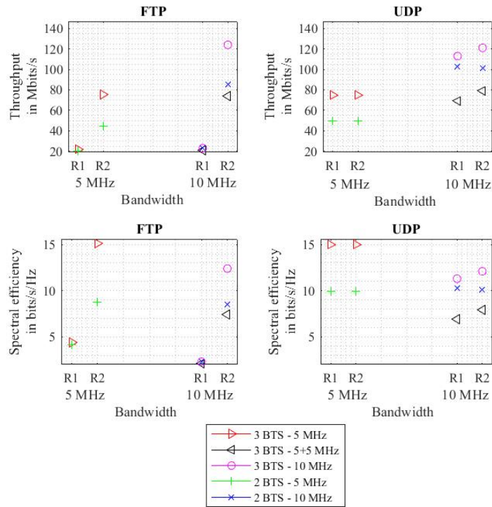
Fig. 6. Variation in the network throughput and spectral efficiency performance between small and large bandwidth usage in the high transmitted power case.
