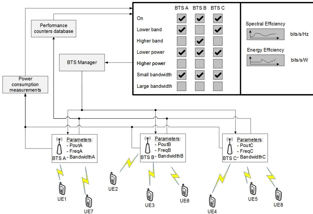
Fig. 2. High level specification of the measurements with all the building blocks involved.
