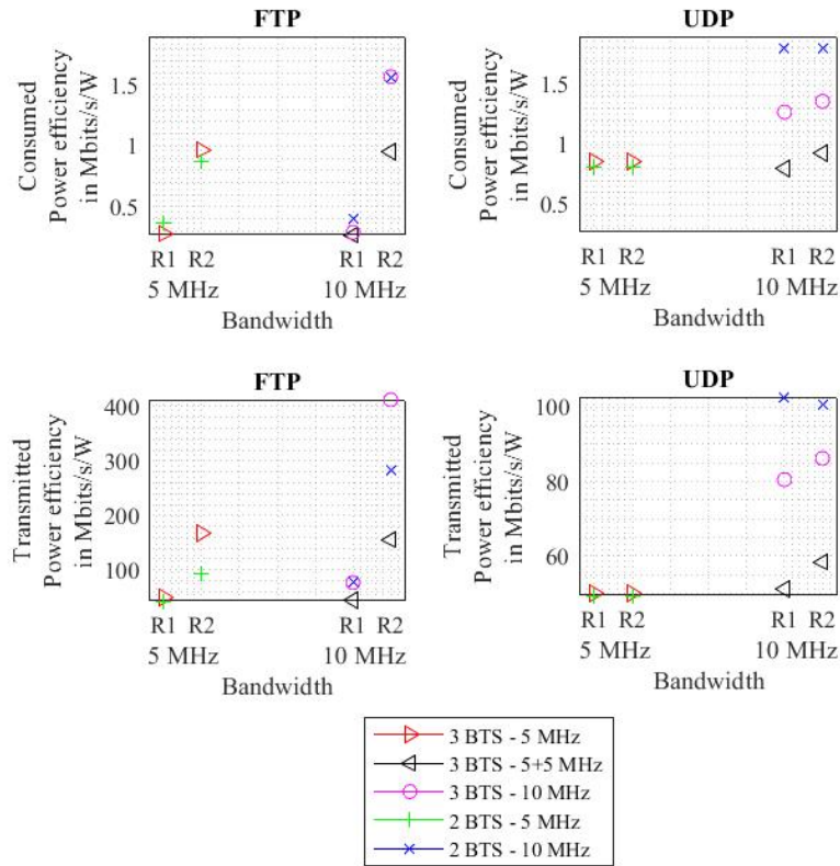
Fig. 7. Variation in the network power efficiency performance between small and large bandwidth usage in the low transmitted power case.
