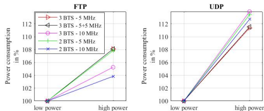
Fig. 3. The variation is in percentage for the power consumption, when the 100 % reference is the low power value for the same test case.
