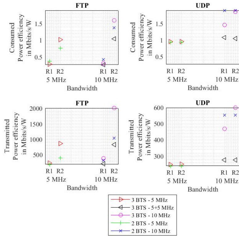
Fig. 7. Variation in the network power efficiency performance between small and large bandwidth usage in the low transmitted power case.
