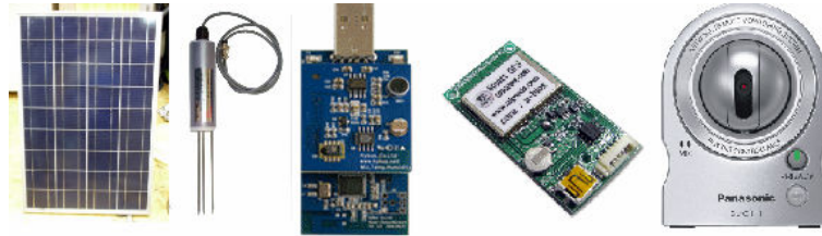
Fig. 7. Solar cell, soil sensor, network sensor node, GPS module and CCTV camera in the FMSS
