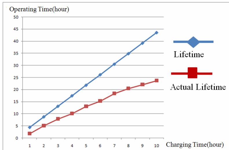
Fig. 13. Comparing estimated lifetime with actual lifetime of the system
