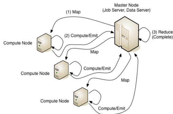
Fig. 1. High Level Map Reduce Explanation
