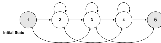
Fig. 2. HMM Topology
