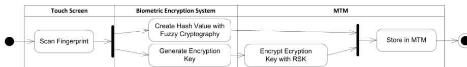
Fig. 2. Setup Process
