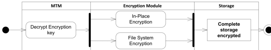
Fig. 3. Encryption Process
