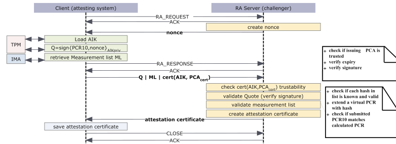
Fig. 2 Flow of the RA protocol
