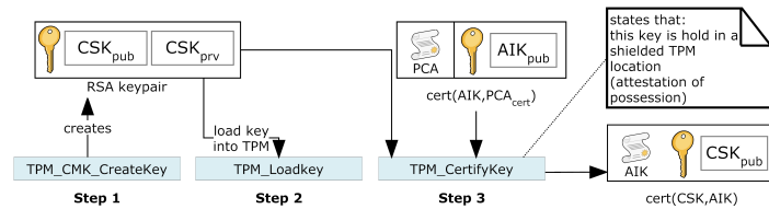
Fig. 3 Creation of the Certified Signing Key (CSK)
