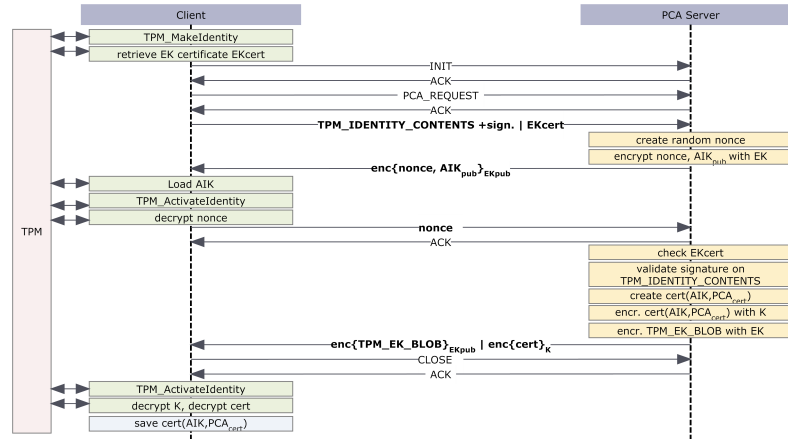
Fig. 1 Flow of the AIK certification protocol
