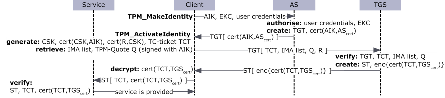
Fig. 5 Protocol of a TC enabled Kerberos Infrastructure
