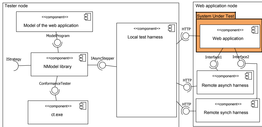
Fig. 1. A SysML component diagram of the setup of model-based testing of a web application.
