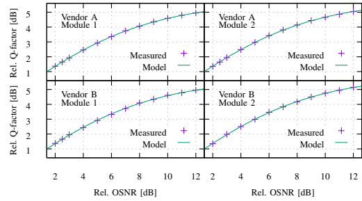
(b) CFP2-DCO modules.
