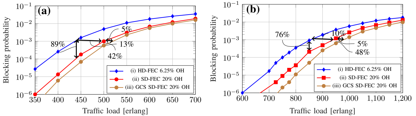
Fig. 1: Blocking probability as a function of traffic load for: (a) NSFNET topology and (b) EUROCORE topology.
