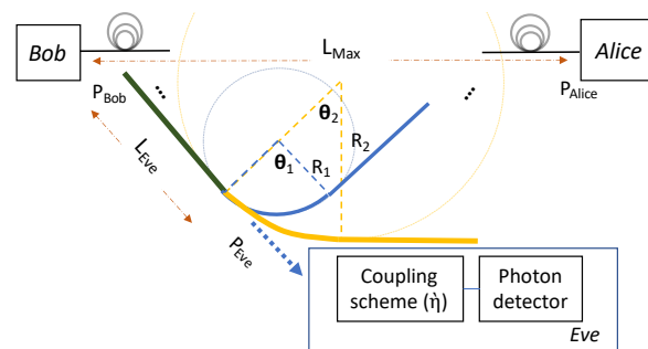
Figure 2. The principle of out-coupling light due to fibre bending at different radii and angles.
