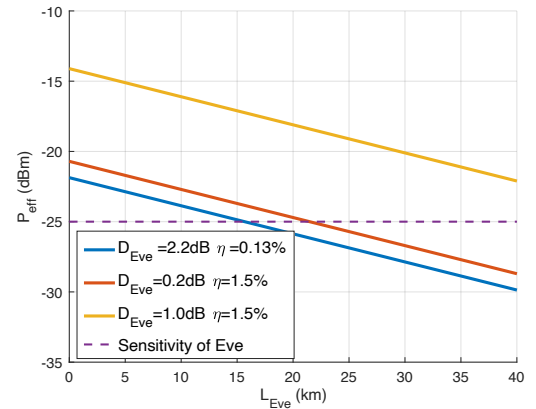
Figure 3. Input power at the Eve's detector ( P_{eff} ) when using eavesdropping devices with different attenuation ( D_{Eve} ) and coupling efficiency ( \eta ).
