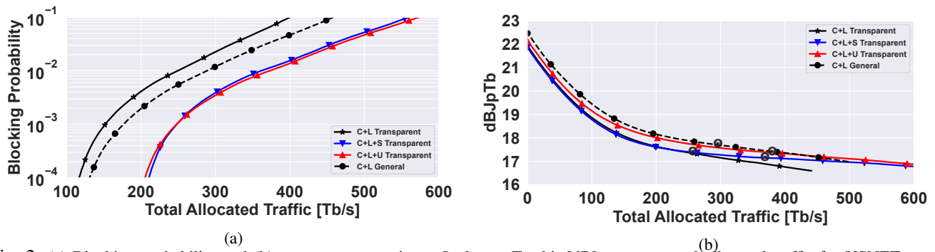
Fig. 2: (a) Blocking probability and (b) energy consumption – Joule per Terabit [dB] – versus total allocated traffic for USNET topology for translucent (C+L-band) and transparent (C+L-, C+L+S-, C+L+U-band) network designs.
