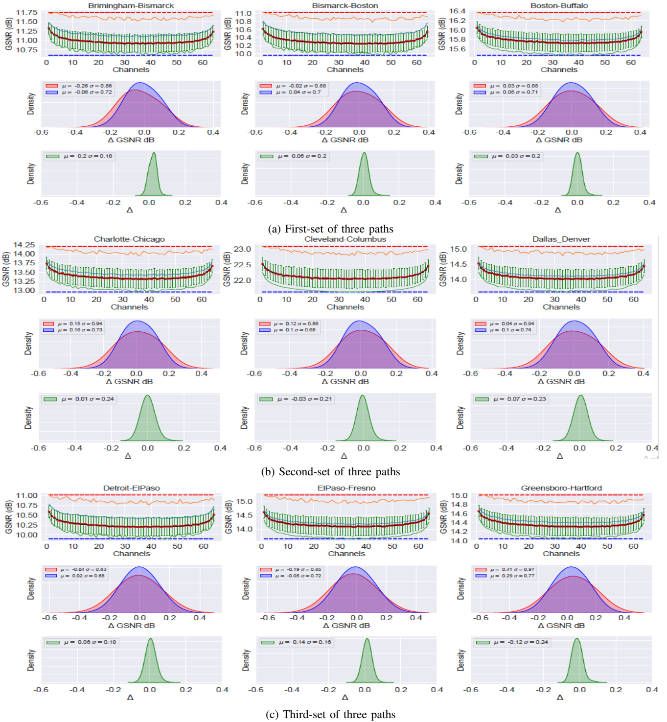
Fig. 2: GSNR statistics ( I^{st} row of each set), \Delta GSNR actual/predicted distribution ( 2^{nd} row of each set), Prediction error ( \Delta ) ( 3^{rd} row of each set): USA Network Paths
