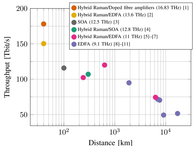
Fig. 1. Record data throughput versus distance for single mode fibre, not including spectral gaps between amplifier gain bandwidths [1].
