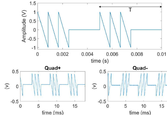
Figure 2: (upper) Time-interleaved DC bias dither signal. (lower): MZ biased a quadrature, with positive slope (left) and negative slope (right).
