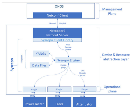
Figure 3: SDN architecture for legacy devices.
