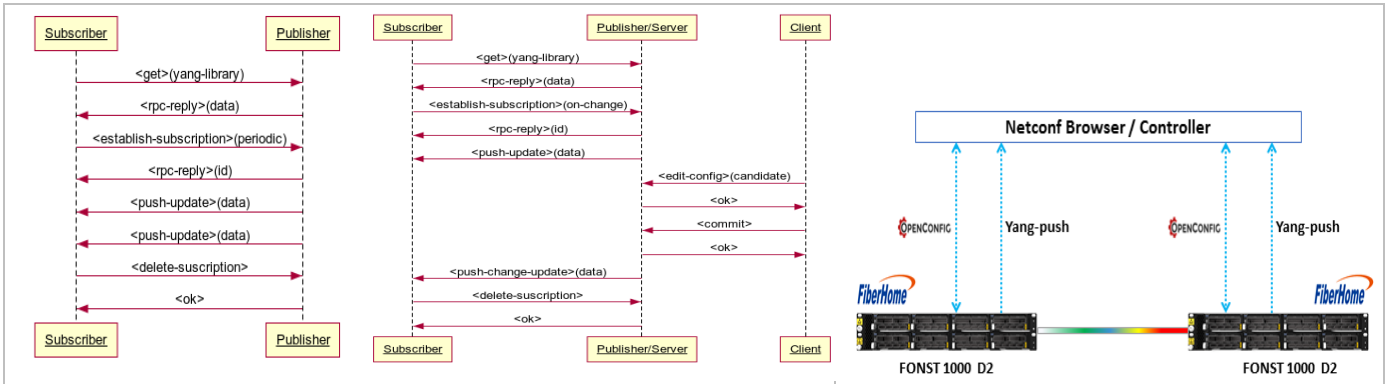
Fig. 2. Periodic Subscription
