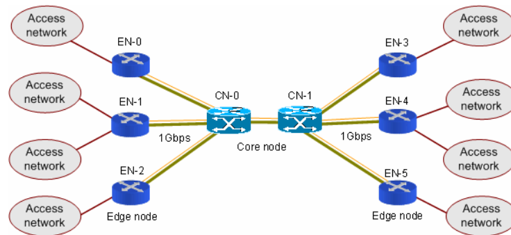
Fig. 4. Network simulation topology with 2 CNs and 6 ENs.
