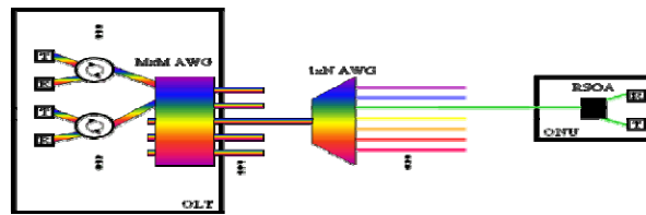
Fig. 5. Dense WDM PON with Reflective ONU
