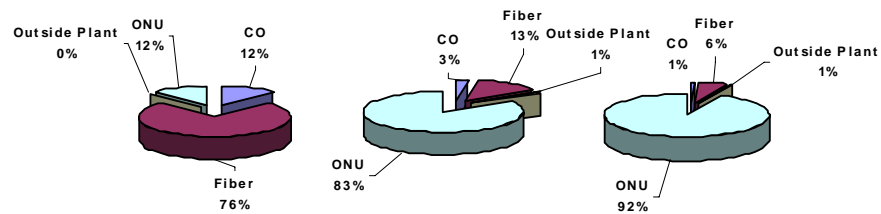
Fig. 9. Contribution to the total cost by each part of the network. Left: P2P Network, Center: TDM PON Network, Right: SARDANA
