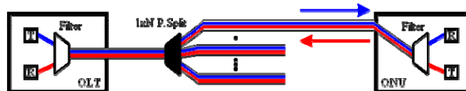
Fig. 3. Single Fiber TDM PON
