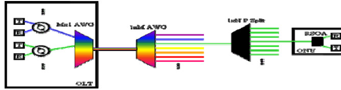
Fig. 4. Coarse WDM PON with Reflective ONU
