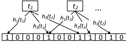
Fig. 1. An example Bloom Filter with m = 12 , and l = 3 .
