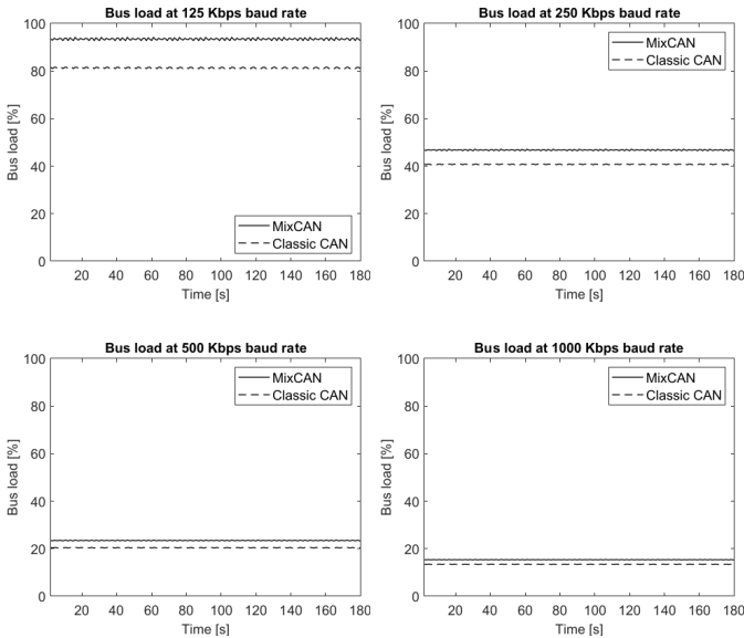
Fig. 4. MixCAN’s impact on the bus load in relation to the configured baud rate.
