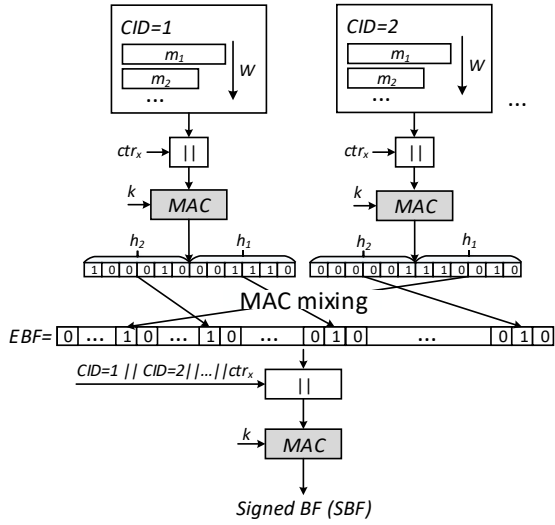
Fig. 2. MixCAN's architecture.
