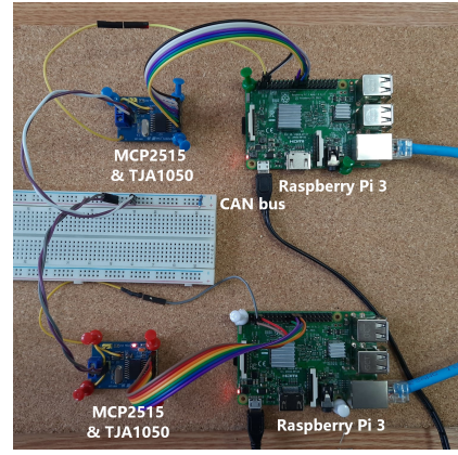
Fig. 5. Experimental test bed ( Scenario B ), including two Raspberry Pi 3 Model B+ boards as ECUs, two CAN controllers and a CAN bus (breadboard).
