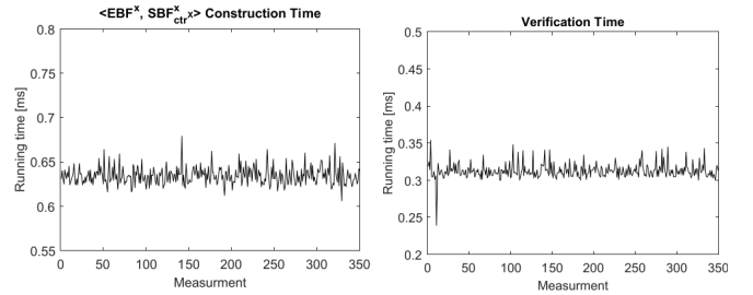
Fig. 7. MixCAN’s computation time in a real test bed comprising two Raspberry Pi 3 Model B+ boards equipped with CAN communication interfaces.
