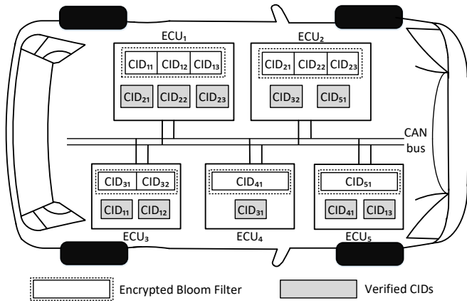
Fig. 3. Experimental setting ( Scenario A ) including ECUs, transmitted encrypted BF, and verified CIDs.
