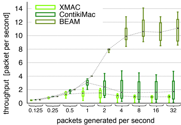
Fig. 18: Maximum throughput.
