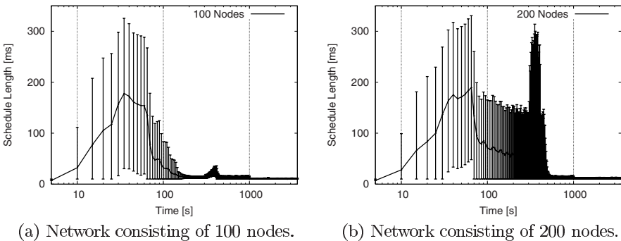
Fig. 5. Average schedule length evolution over the first hour (log-scaled)
