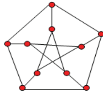
Fig. 2. Petersen graph
