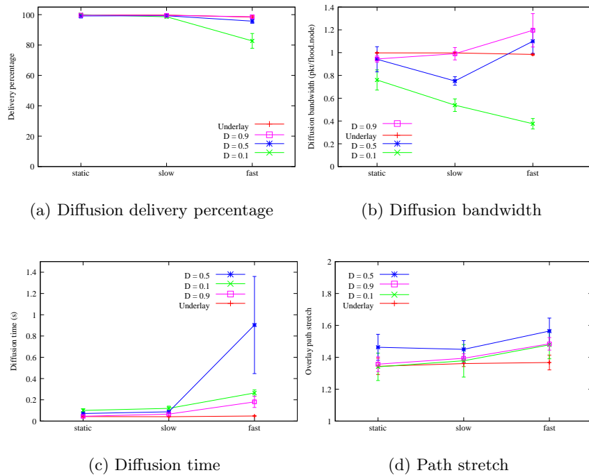
Fig. 3. Overlay flooding performance over OLSR
