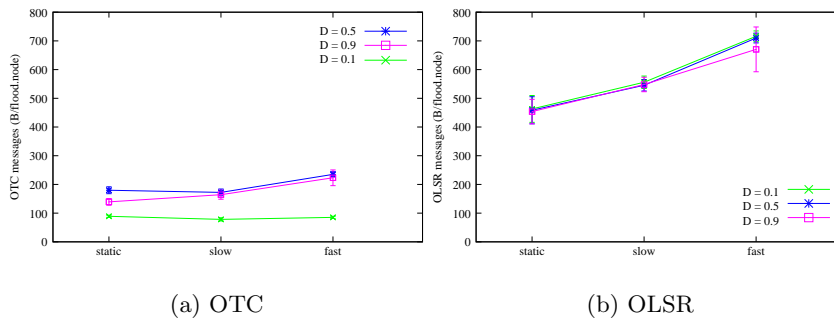
Fig. 4. Comparison of the bandwidth consumed by OTC and OLSR
