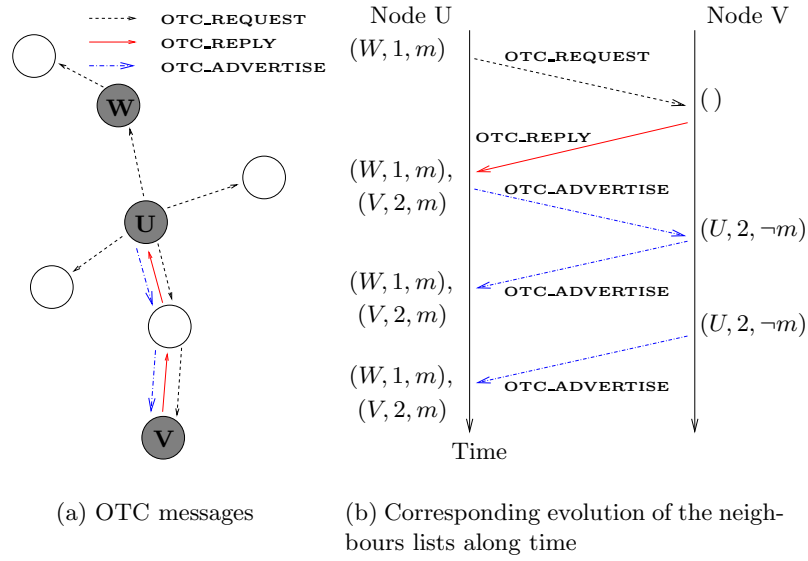
Fig. 1. Discovery procedure
