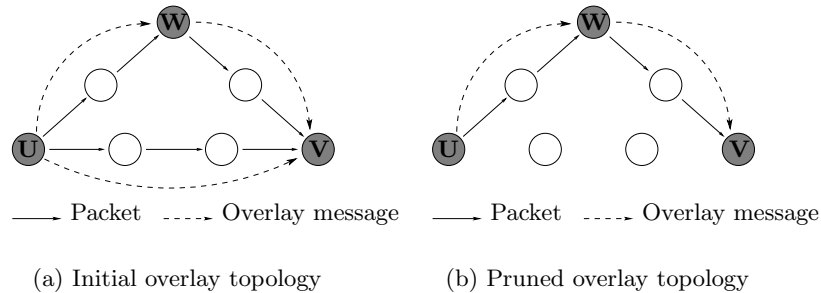
Fig. 2. Diffusion consumes less bandwidth on the pruned overlay topology
