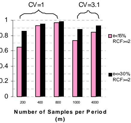
Figure 4: Quantitative Accuracy
