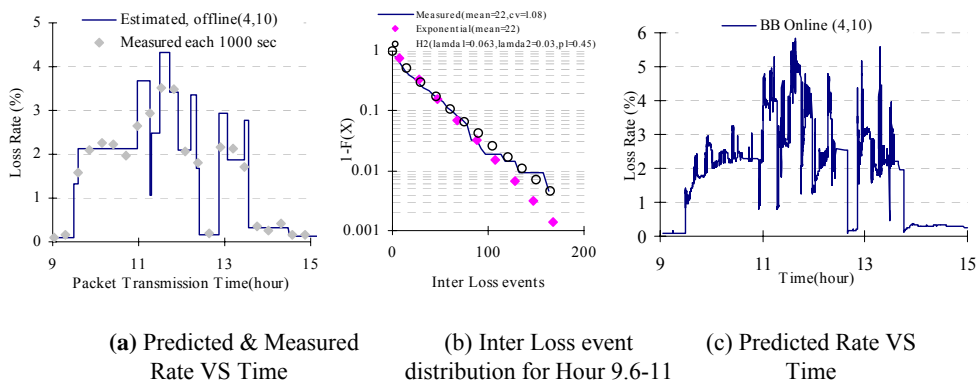
Figure 6: Actual & BBA Predicted Loss Rate
