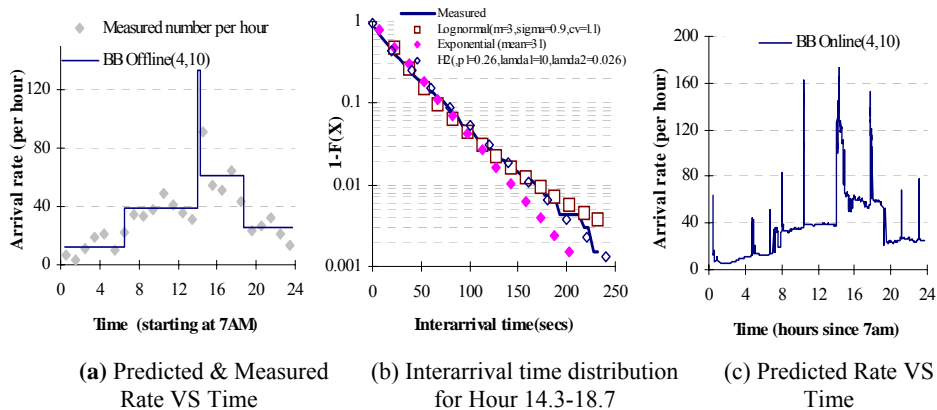
Figure 5: Actual & BBA Predicted Media Server Request Arrival Rate
