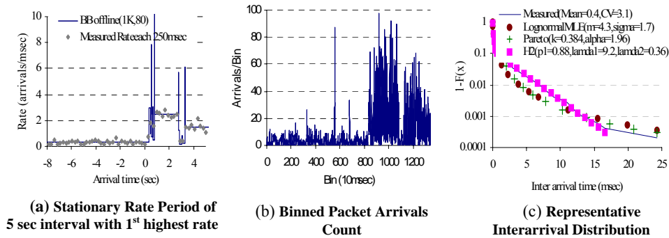
Figure 7: BBA on IPEX Gateway Trace
