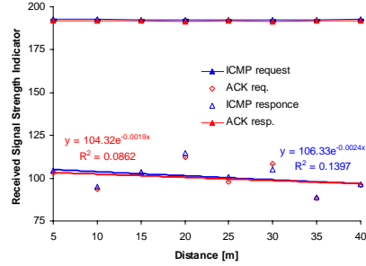
Fig. 5. Received signal strength indicator versus distance. Confidence intervals are too small to be shown.
