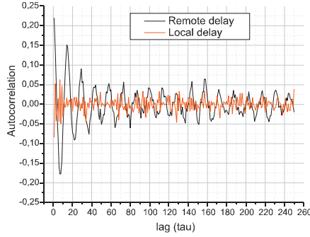
Fig. 7. Autocorrelation (=cross correlation of itself) is oscillating for remote delays – indicating a fundamental frequency component in observations (at 40 m).
