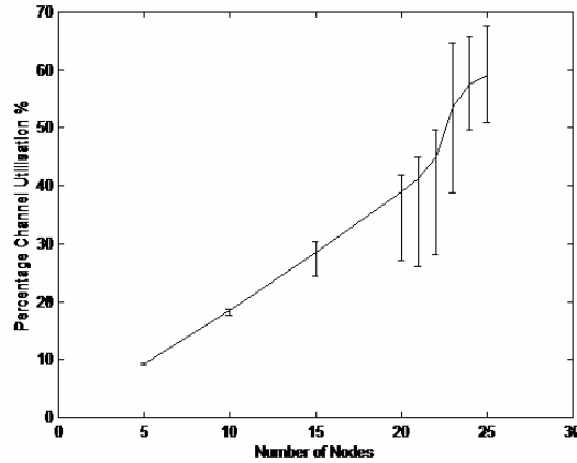
Figure 3 - Channel Utilisation (In the 12Mbps case)
