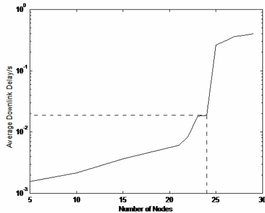
Figure 2 - End-to-End delay for varying number of 54Mbps calls
