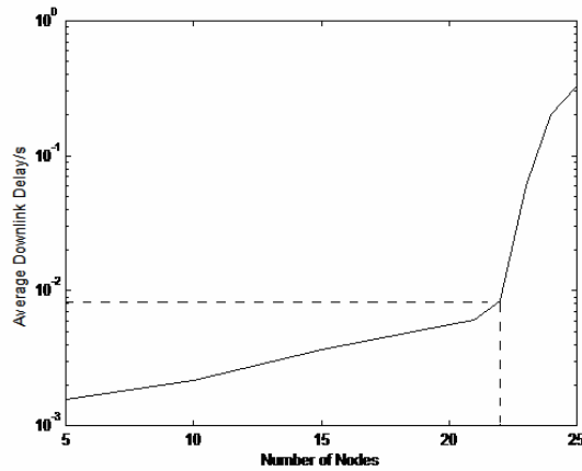
Figure 4 - End-to-End delay (In the 12Mbps case)
