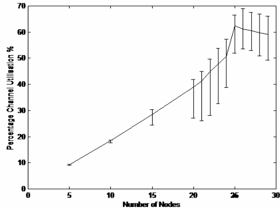
Figure 1 - Channel Utilisation for varying number of 54Mbps calls
