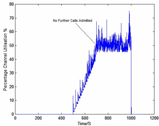
Figure 5 - Heterogeneous Data Rate Simulation
