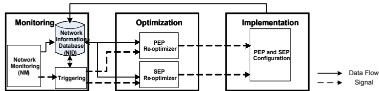
Figure 1. Inter-domain Outbound Traffic Engineering Framework
