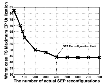
Figure 2(b). SEP Reconfiguration limit
