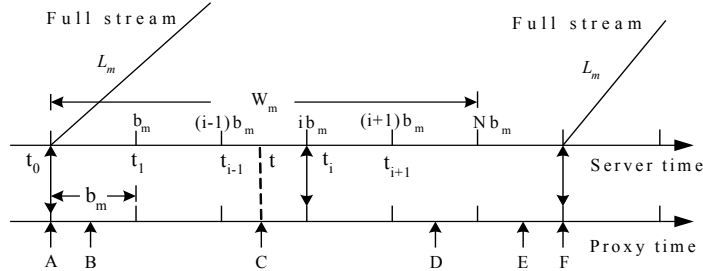
Fig. 2. Timing Diagram for adaptive batched patch caching
