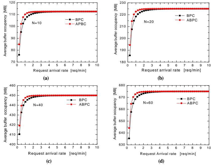
Fig. 5. Average buffer occupancy at proxy versus request arrival rate at different values of patching window, b_m=1 [min]
