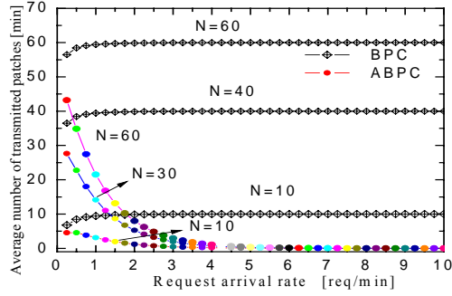
Fig. 3. Average number of transmitted patches through extra channel versus the request arrival rate, b_m=1[\text{min}]
