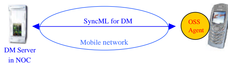
Fig. 1. Mobile agent based monitoring architecture
