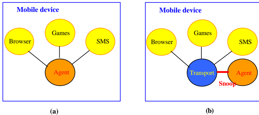
Fig. 2. An agent inside a mobile device
