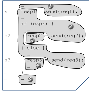
Fig. 8. Code slicing for continuations
