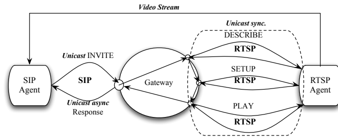
Fig. 1. SIP to RTSP gateway
