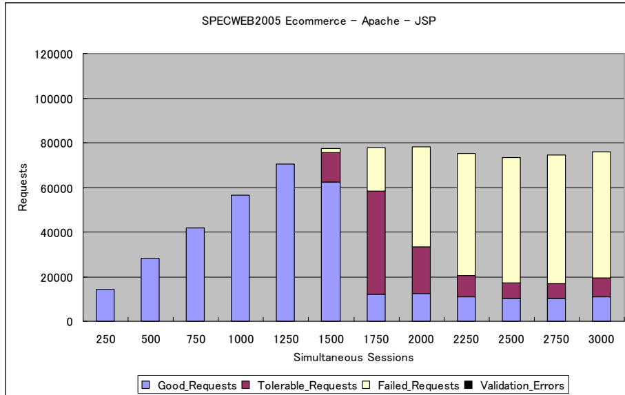
Fig. 8. SPECweb2005 Ecommerce Performance with JSP and Apache
