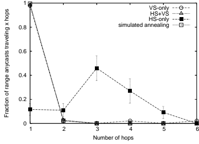
Fig. 7. Range Anycast: Hops required to delivery when sending from MID to range [0.85, 0.95].
