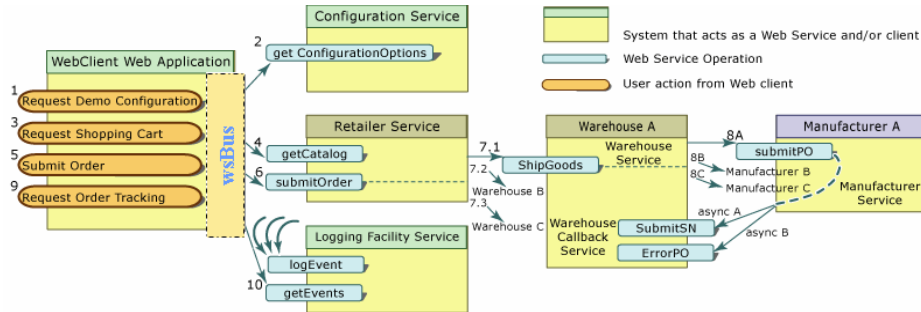
Fig. 4. WS-I Supply Chain Management (SCM) application process (adapted from [17])
