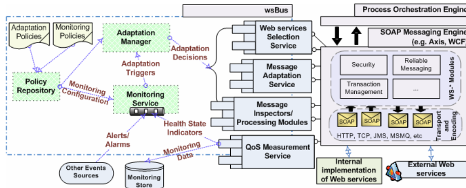
Fig. 3. wsBus Architecture
