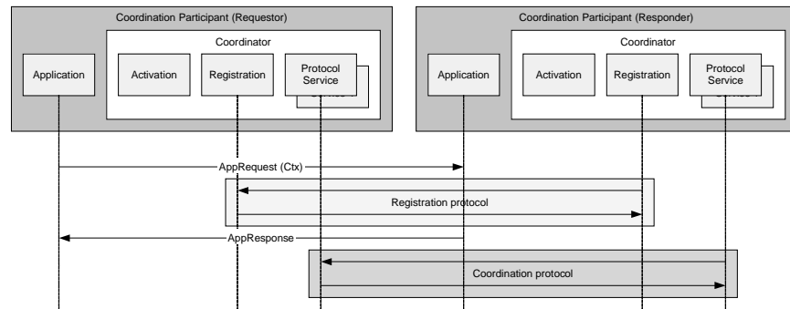
Fig. 3. WS-Coordination Architecture
