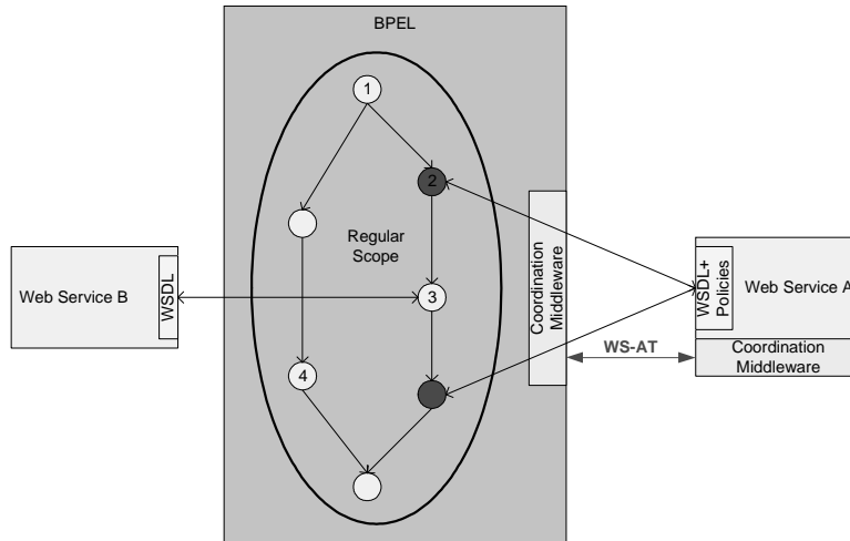
Fig. 4. Coordinated partner links in regular scopes: Attaching a WS-AT policy on a PartnerLink connecting the process with Web Service A and required coordination middleware for WS-AT protocol interactions
