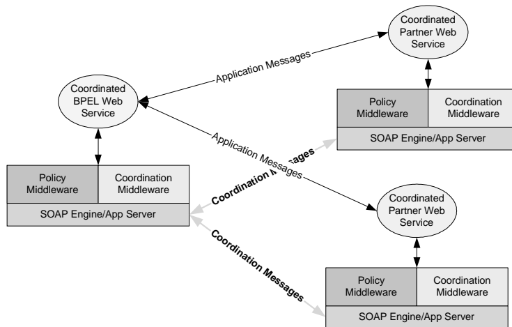
Fig. 6. Middleware prototype: Sample deployment architecture
