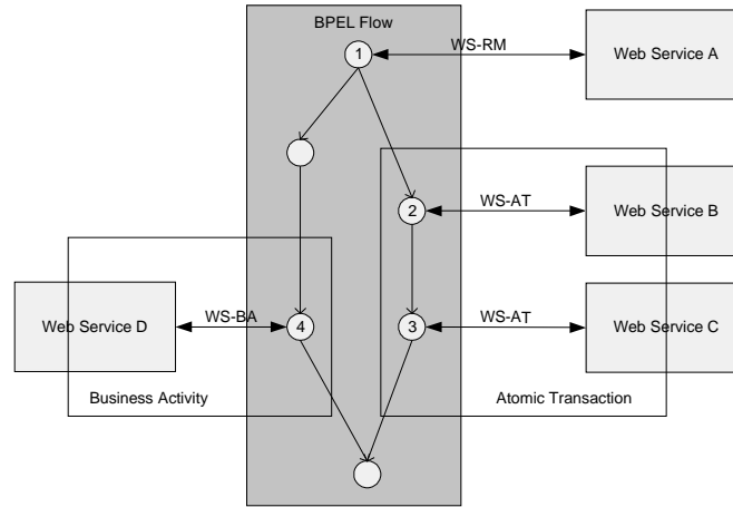
Fig. 2. Coordination requirements for service composition
