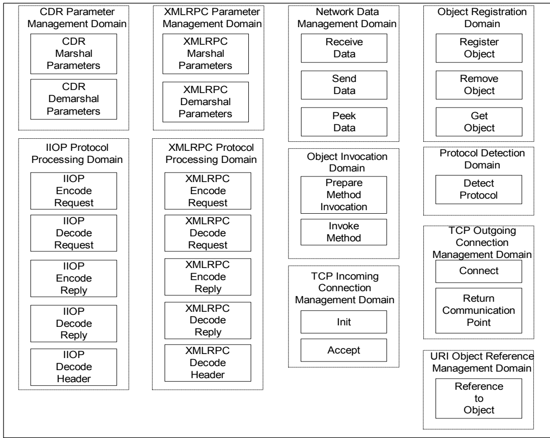
Fig. 10. ExORB structure.
