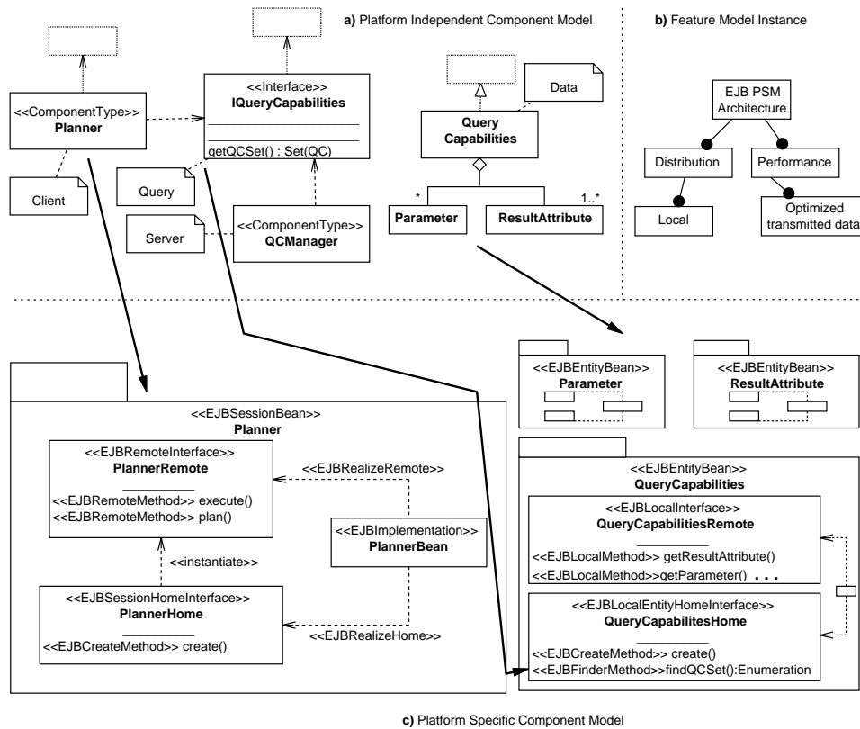
Figure 10. Example - PIM-PSM Transformation for a Local Configuration
