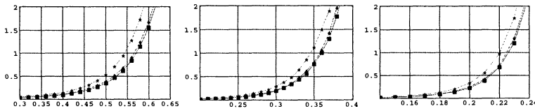
Figure 6. Mean connectivity period length for n = 20, 100, 500 nodes (from left to right) with different velocity distributions.
