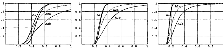
Figure 1. Validation of 1-connectivity for n = 20, 100, 500 nodes (from left to right) as a function of d , dashed lines depict simulations and solid lines analytical results.
