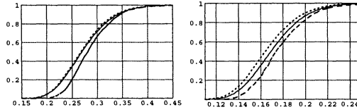
Figure 3. Comparison of the accuracy of A1 (solid lines) and the approximation in [11] (dotted lines) against simulations (dashed lines) for n = 100, 500 (left, right) nodes.
