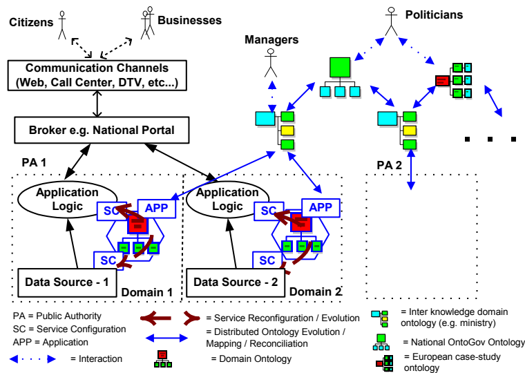
Fig. 3. OntoGov service provision model
