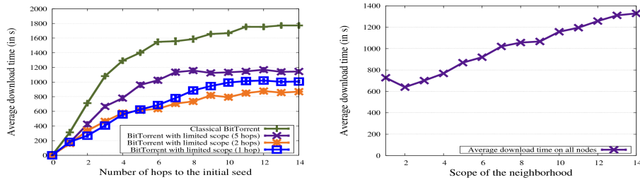
Fig. 1. Download time per peer vs. number of hops to the initial seed Fig. 2. Download time per peer vs. scope of sharing
