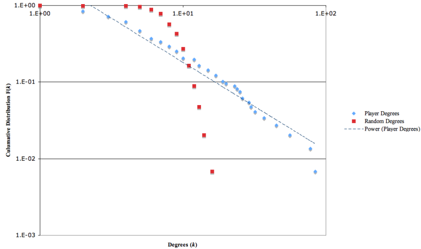
Fig. 1. Cumulative Distribution of Degrees in Familiars and Random Networks
