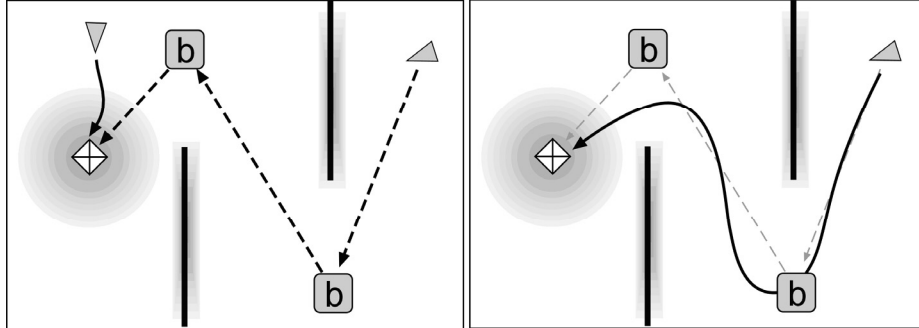
Figure 7. Path solving.
