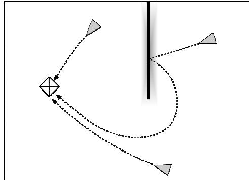
Figure 6. Particle-based navigation.
